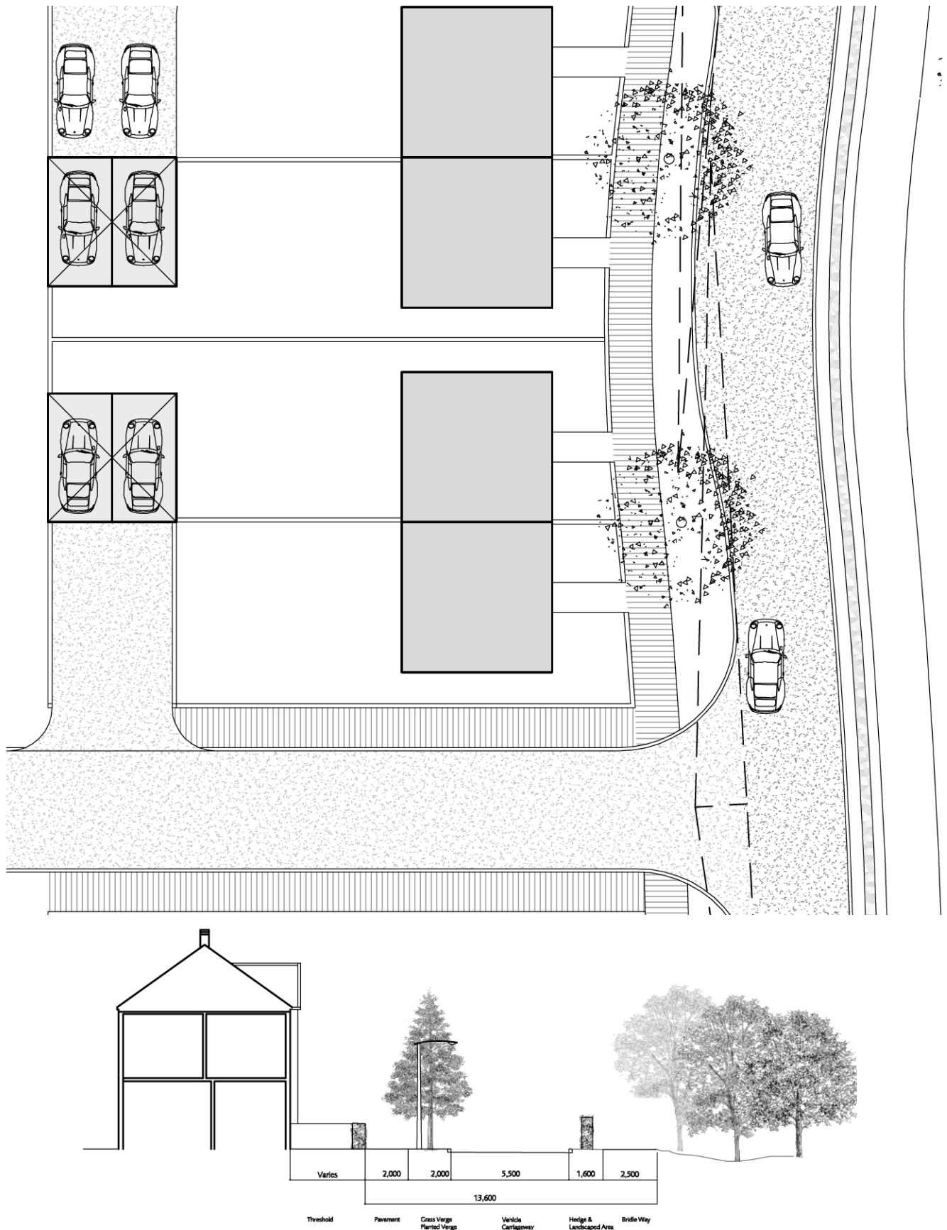
Figure A 6.3 'Farm Lane' - Typical section
