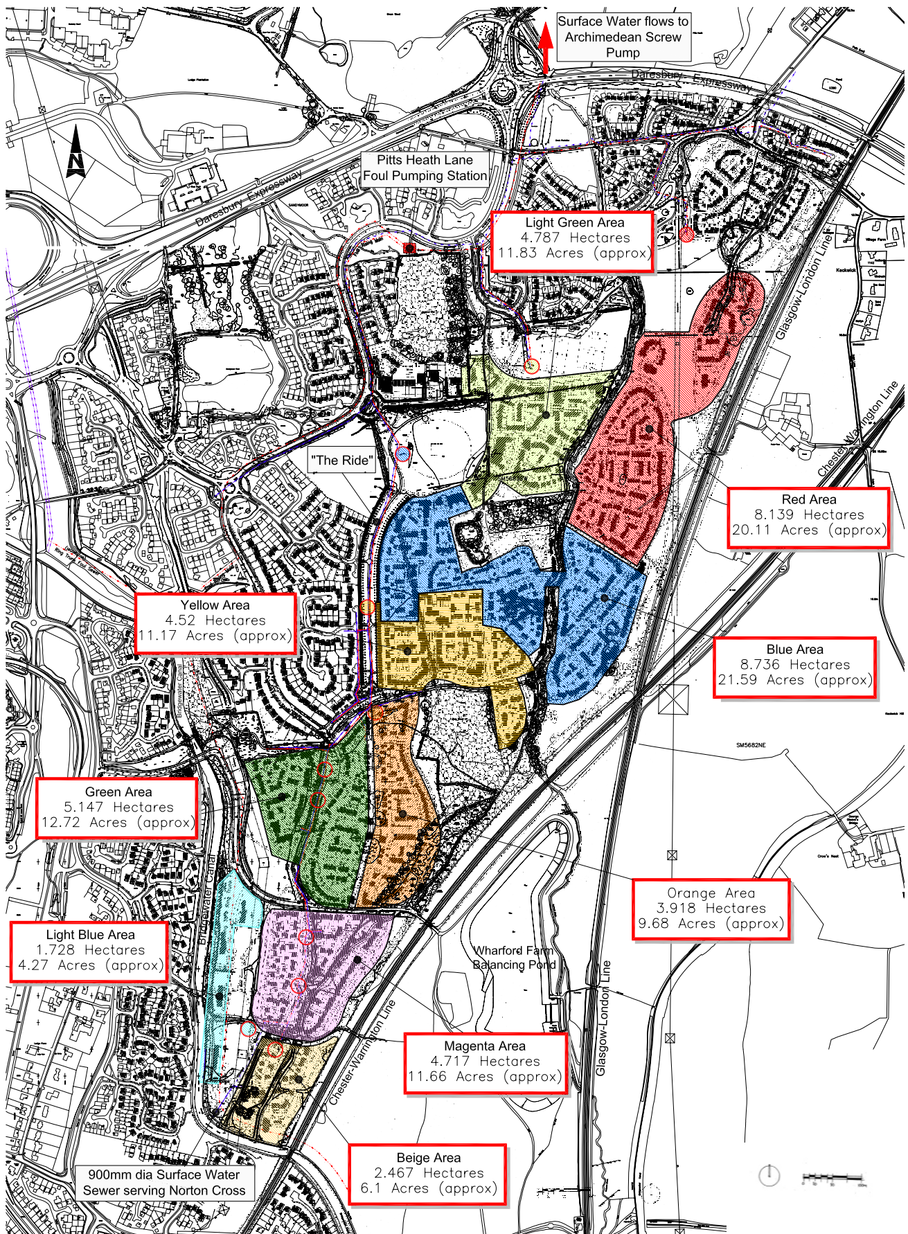
Figure 3.9 Drainage plan
