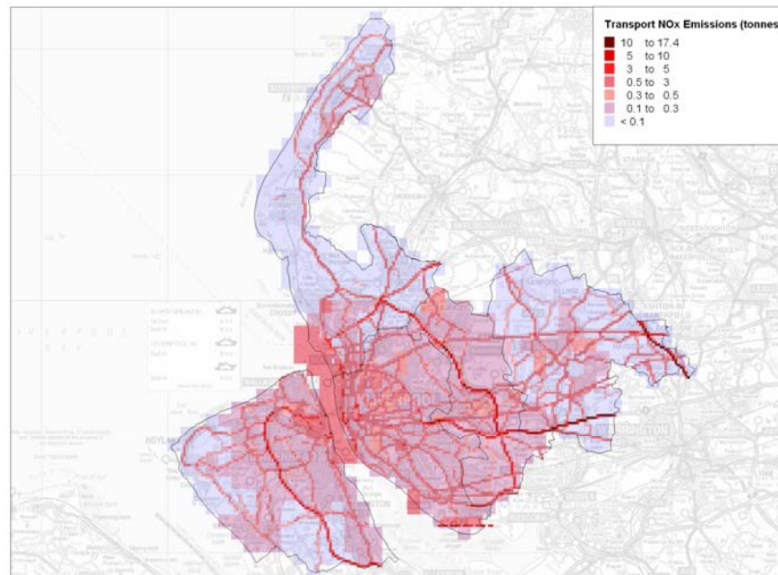
Figure C.11: Transport NO x Emissions for the Liverpool City Region
