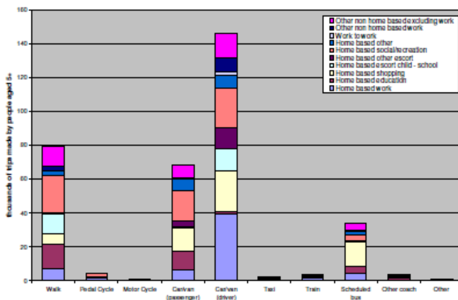
Figure C.35: 2010 Main Mode by Overall Purpose (Halton)
